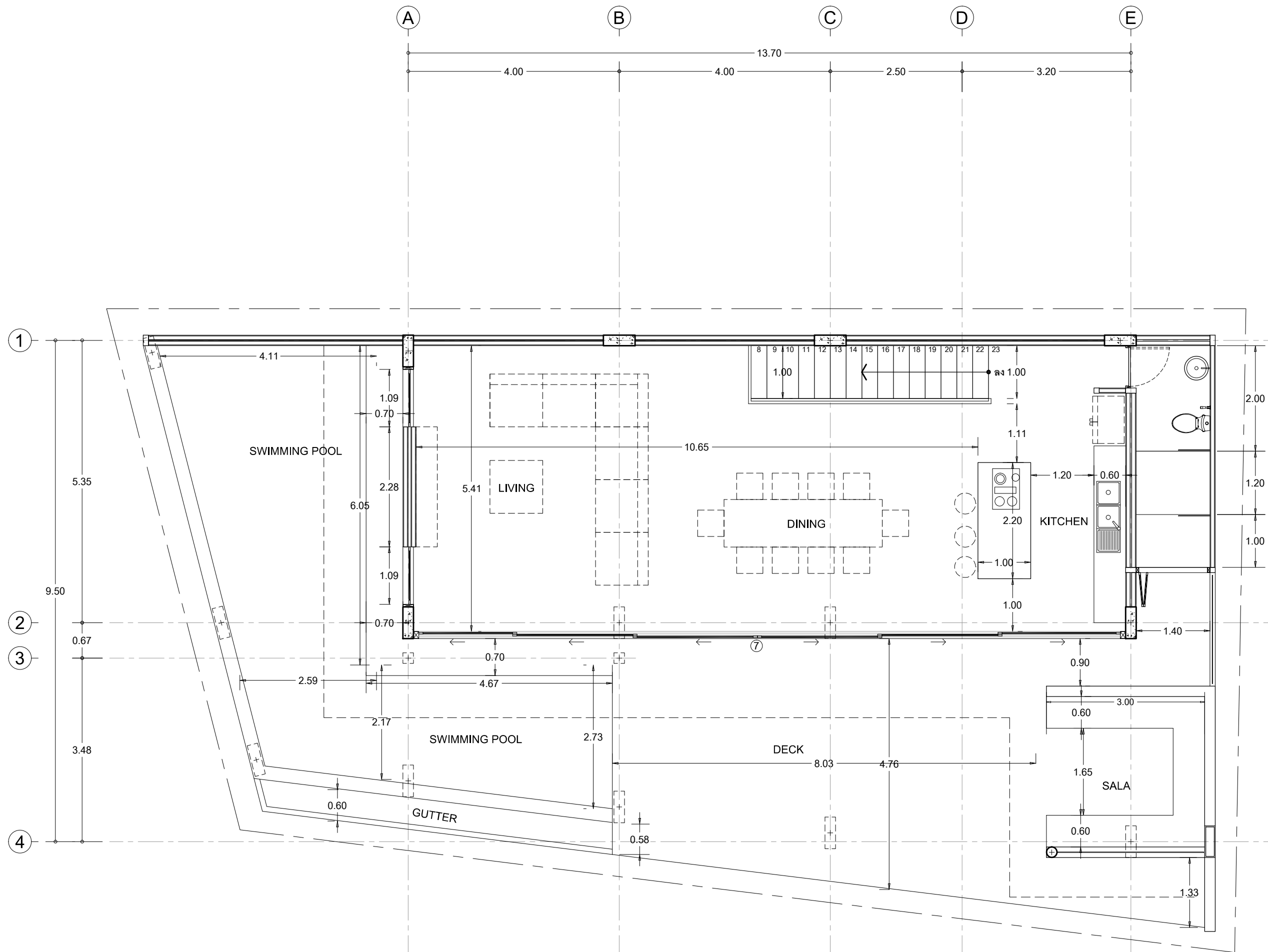
ARI VILLA THIRD FLOOR PLAN
